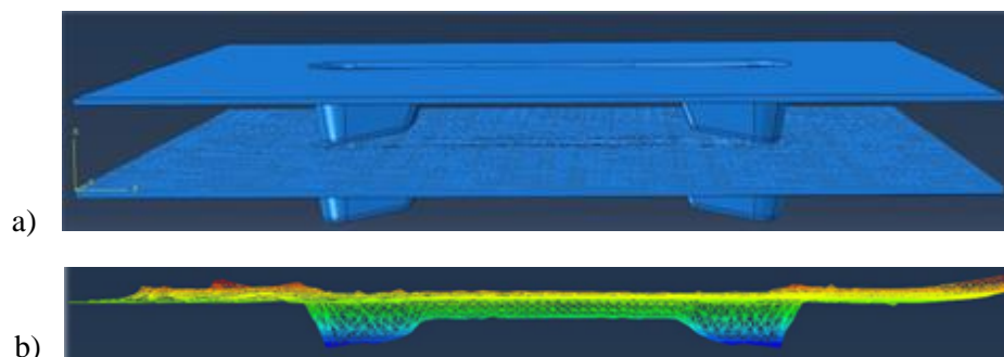
Figure 2. Forming simulations at the design stage: a) matching moulds with flat fabric in between, b) side view of the deformed fabric.
