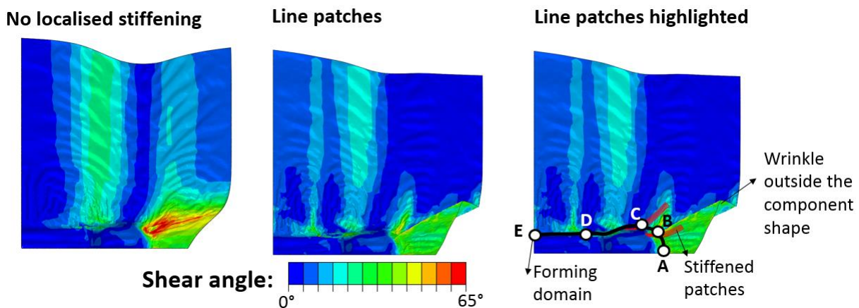
Figure 7. Forming simulations with and without stabilising patches
