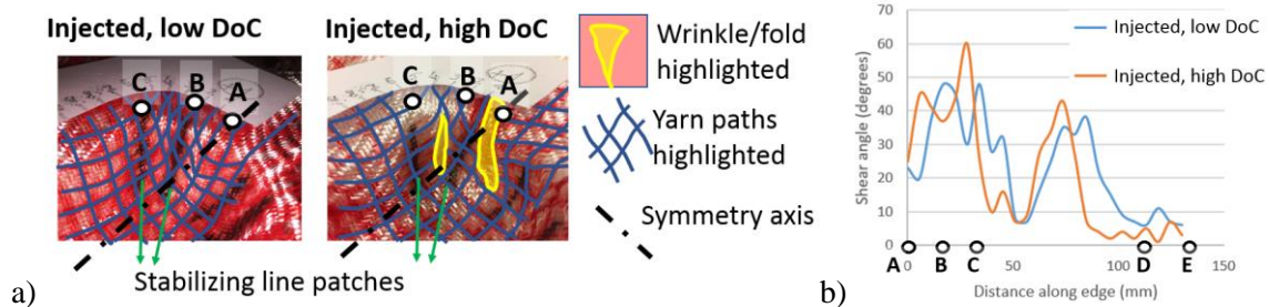
Figure 6. a) Deformation of the formed fabric with different line treatments, b) Shear angle along the edge A-B-C-D-E (see Fig. 1 for references).
