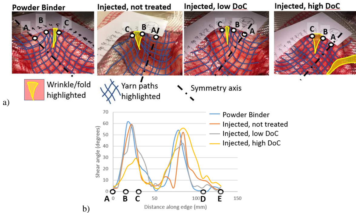
Figure 5. a) Deformation of the formed fabric with different patch treatments, b) Shear angle along the edge A-B-C-D-E (see Fig. 1 for references).
