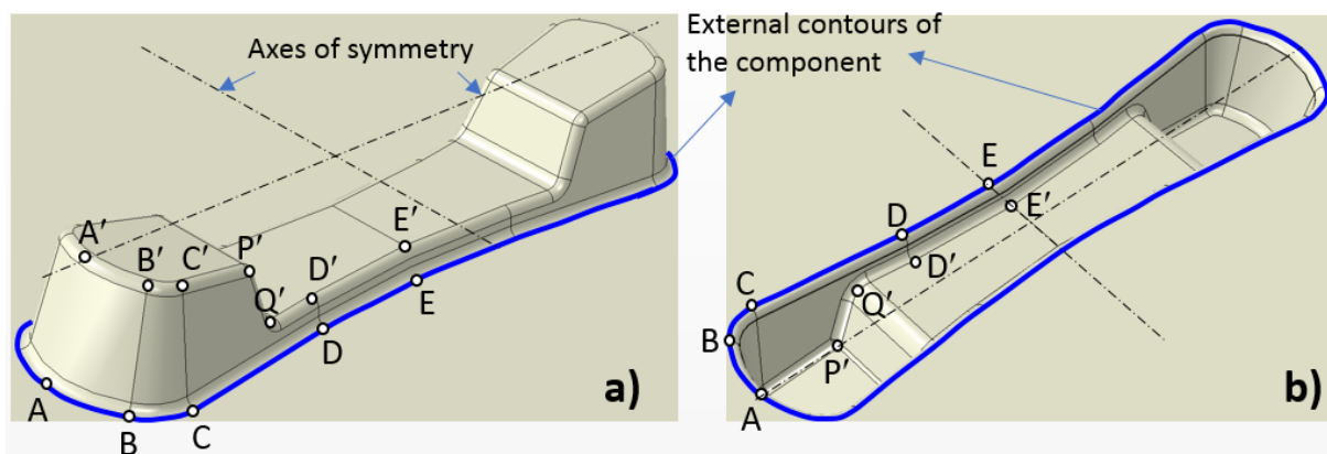
Figure 1. Geometry of the a) male and b) female moulds of the component.
