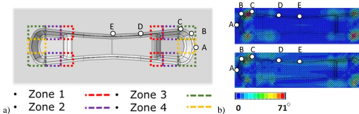
Figure 3. a) Definition of zones for introducing stabilising elements, b) Comparison of shear maps in reference (non-stabilised) and stabilised configurations (zones 3, 4).
