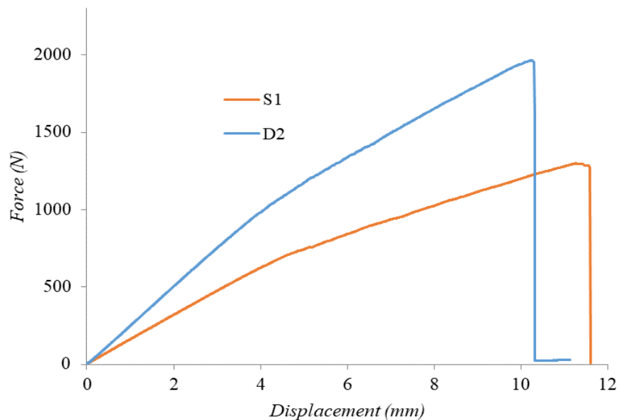
Figure 4. Load/Deflection curve from specimen S1 and D2.
