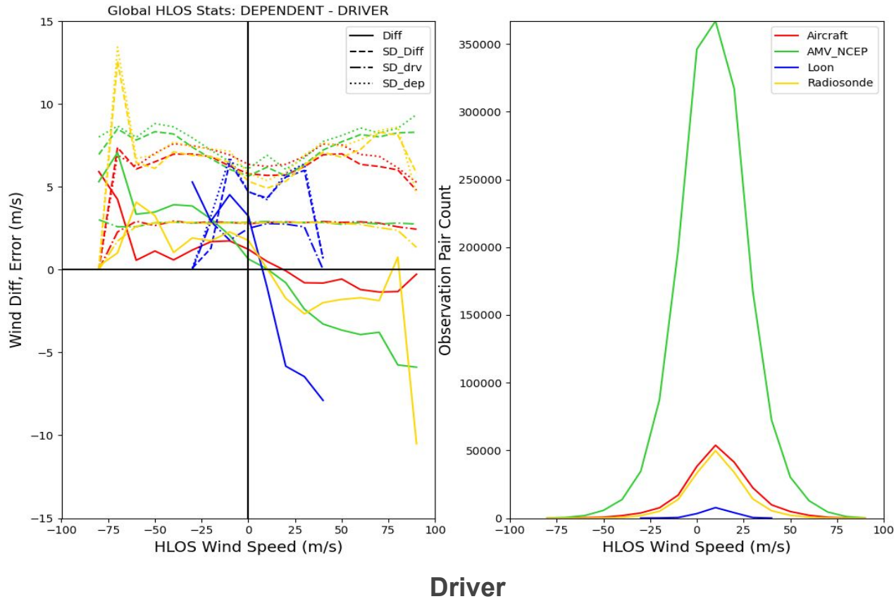
Wind Diff, SD of Diff per Dataset
