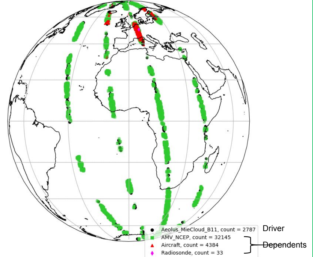
Figure produced from collocation application developed for this project. AMVs, aircraft winds, and rawinsonde winds are collocated with Aeolus Mie-cloudy winds from 2 nd reprocessed campaign.
