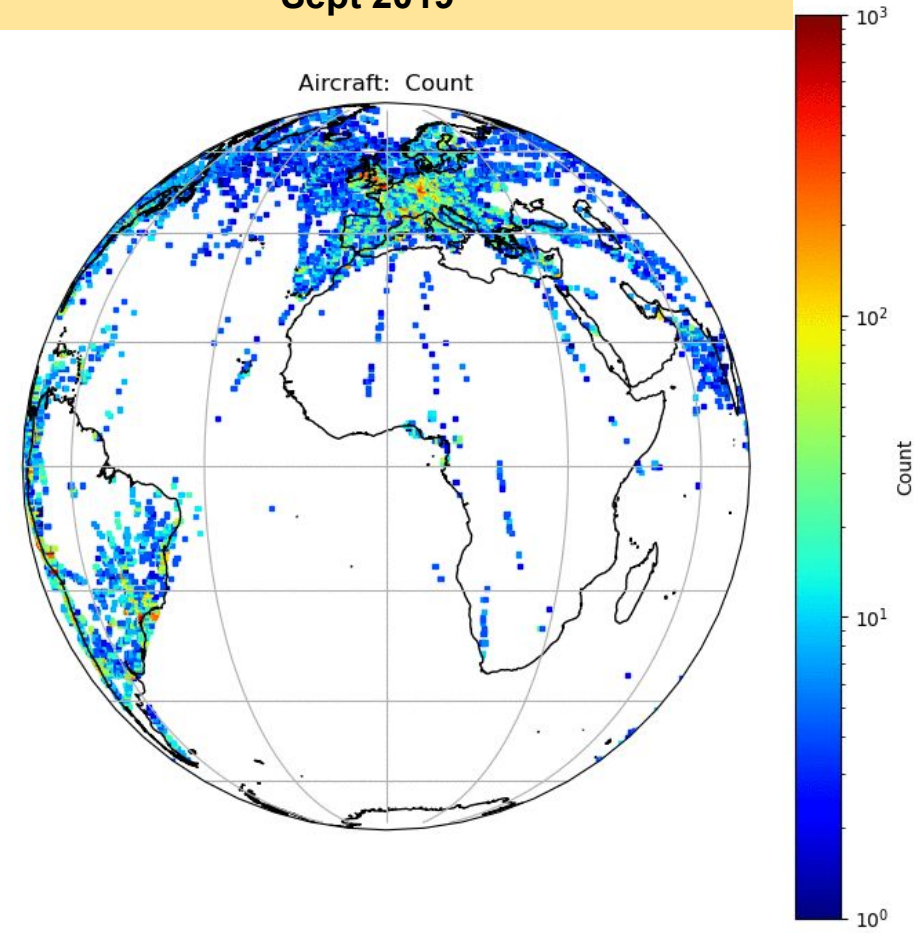
Aircraft Observation Density (i.e., Counts) collocated with Aeolus Rayleigh-clear Sept 2019
