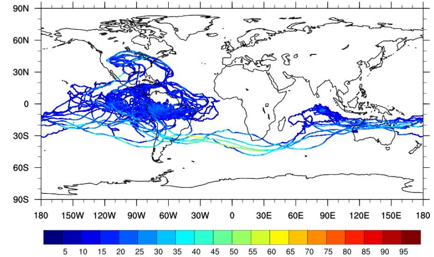
Loon wind speed at all levels, 2019-09-01 00UTC to 2019-12-31 18UTC
