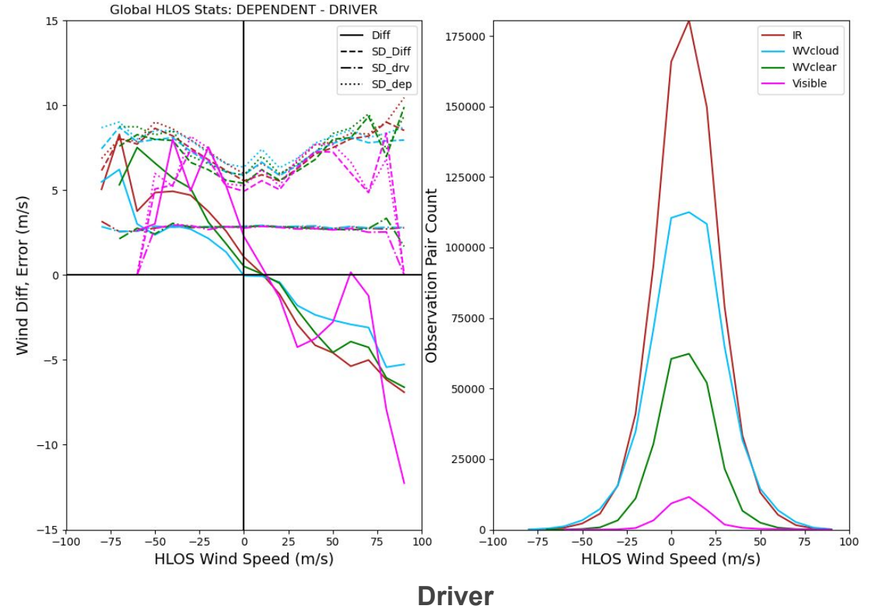
Wind Diff, SD of Diff per AMV type
