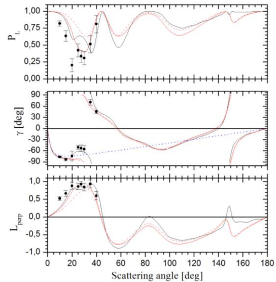
Figure 2. EICP ( P_L , \gamma , L_{\text{perp}} ) for electronic excitation (80 eV) of 4^1P_1 Zn state. Experimental data ( \bullet ) are presented together with (—) CCC, (—) RDWA, (---) SC RDWA and (···) FBA theoretical predictions [4,14].
