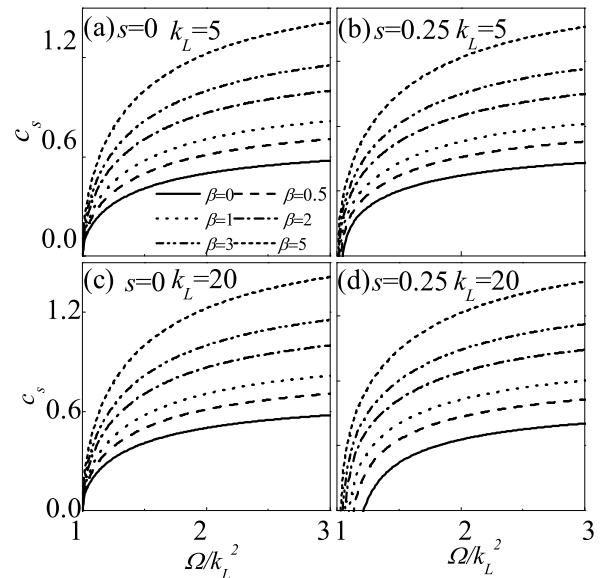
Figure 1. Sound speed against Raman coupling for different atomic interaction in zero momentum phase regime
