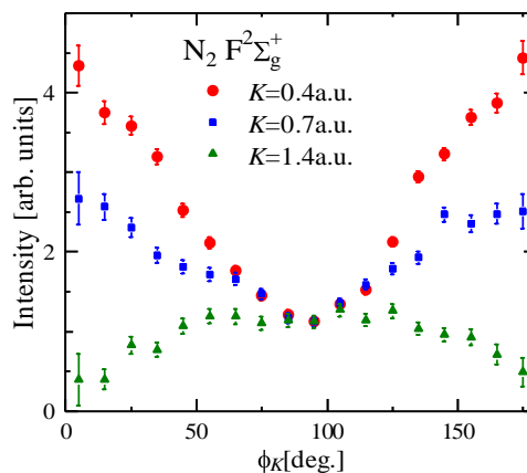
Figure 1. Molecular frame EELS cross section of N 2 for the transition to the F 2 Σ g + state.
