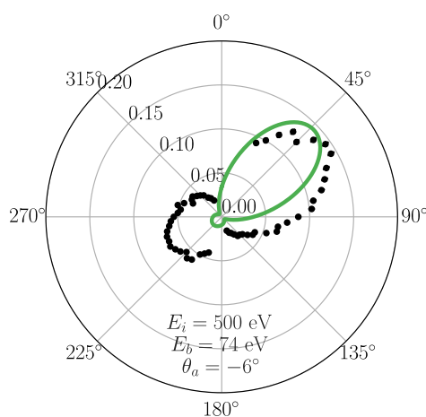
Figure 1. TDCS for NH 3 ( 3a_1^{-1} ). The kinematic conditions are: incident electron energy E_i = 500 eV, ejected electron E_b = 74 eV. The scattered electron is detected at \theta_a = -6^\circ . Experimental data from [10].
