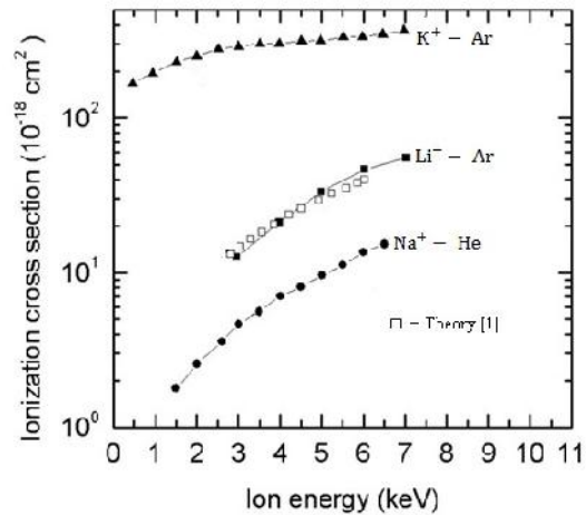
Figure 1. Dependences of the absolute ionization cross section on energy of ions
