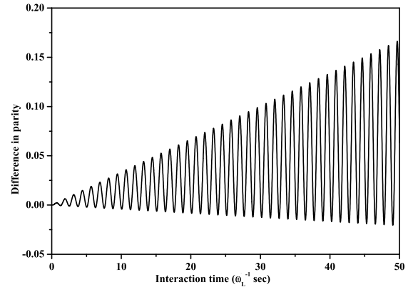
Figure 1. The difference of parity at d = 10^3 a_0 and \omega_L = 1.4 MHz (where, a_0 is Bohr radius and \omega_L is spin Larmor frequency) with \vec{B} = 0.1 mT.
