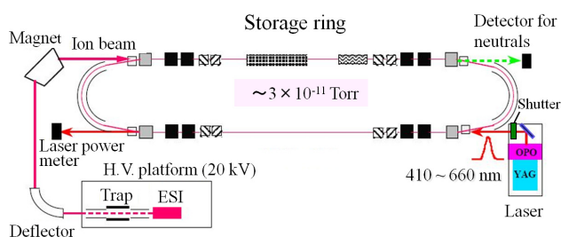
Fig. 2 Experimental setup.
