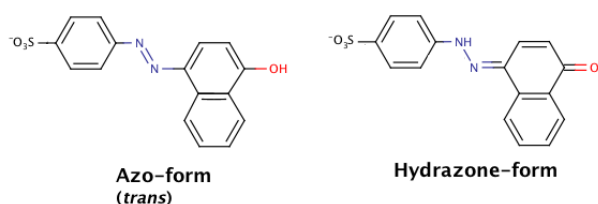
Fig. 1 Chemical structures of orange I monoanions.
