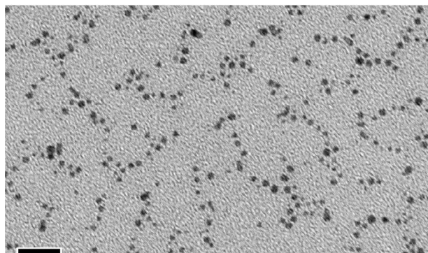
Figure 1. Representative TEM image, showing 50:50 \beta Glc:PEG-amine. Scale bar is 20 nm.
