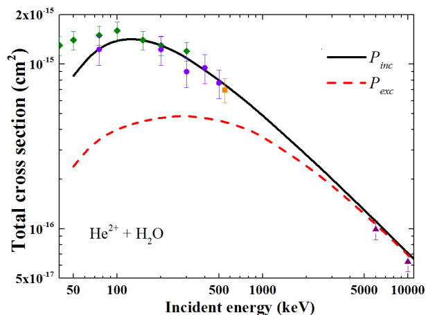
Figure 1. Total single ionization cross sections as a function of the incident energy for \text{He}^{2+} impacting on \text{H}_2\text{O} .
