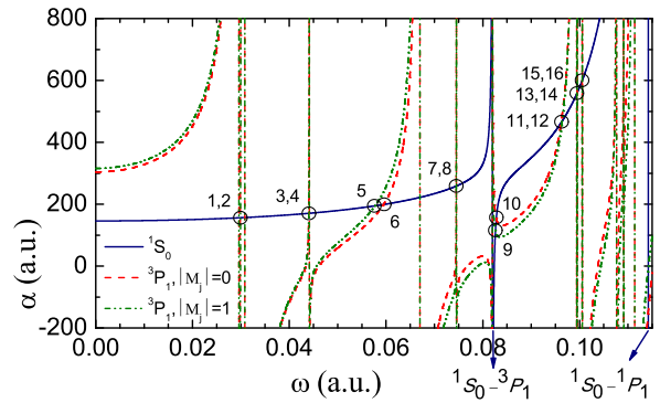
Figure 1. (color online) Dynamic polarizabilities of 6s^2\ ^1S_0 and 6s6p\ ^3P_1 states of Yb atom.
