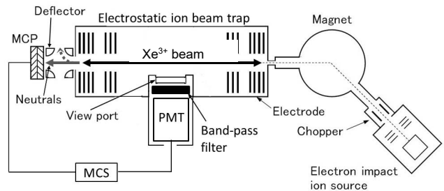
Figure 1. Experimental arrangement
