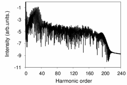
Figure 1. HHG spectra of H_2^+ driven by a 1600-nm laser pulse.
